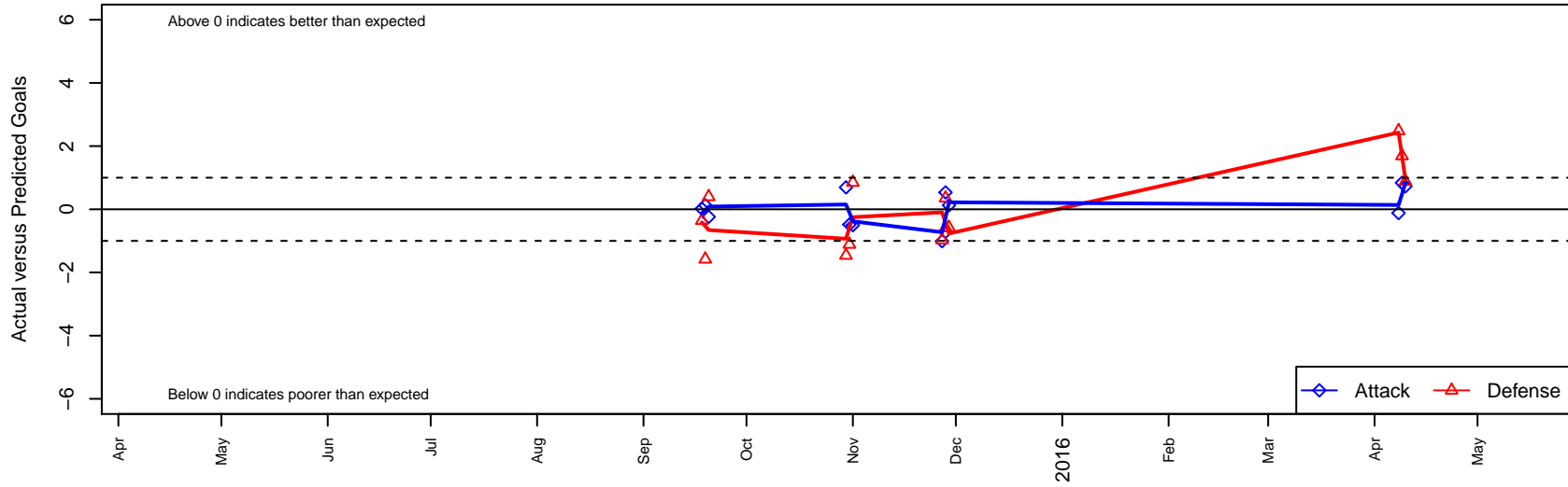
Players SC 02 Elite AP G01 Dots are actual minus expected GF (blue circles) and GA (red triangles). Blue line is smoothed change in attack strength. Red is smoothed change in defense strength.
